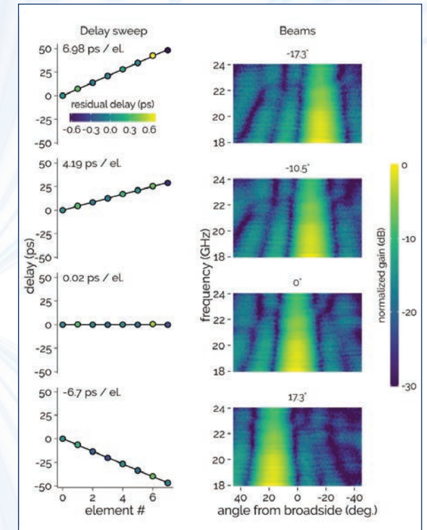
FIGURE 2: Time delay sweep across an 8 – element antenna array (left) and measured receive-mode antenna array patterns (right) for four simultaneous beams.
