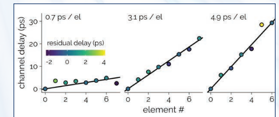
FIGURE 4: Time delay sweep across three integrated optical beamformers similar to that shown in Fig. 3.
