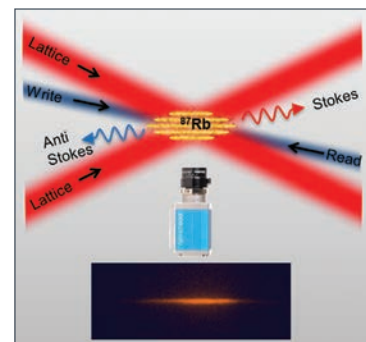
FIGURE 3. Setup for ^{87}\text{Rb} quantum memory in an optical lattice and a fluorescence image of a cloud of ^{87}\text{Rb} atoms confined in an optical lattice.
